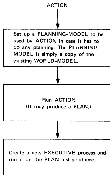
FIGURE 1 SIMPLIFIED FLOW CHART FOR PERFORM
