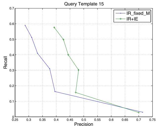
Figure 3: Recall and precision for query template 15.
