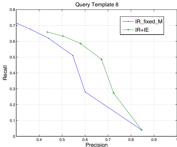
Figure 2: Recall and precision for query template 8.
